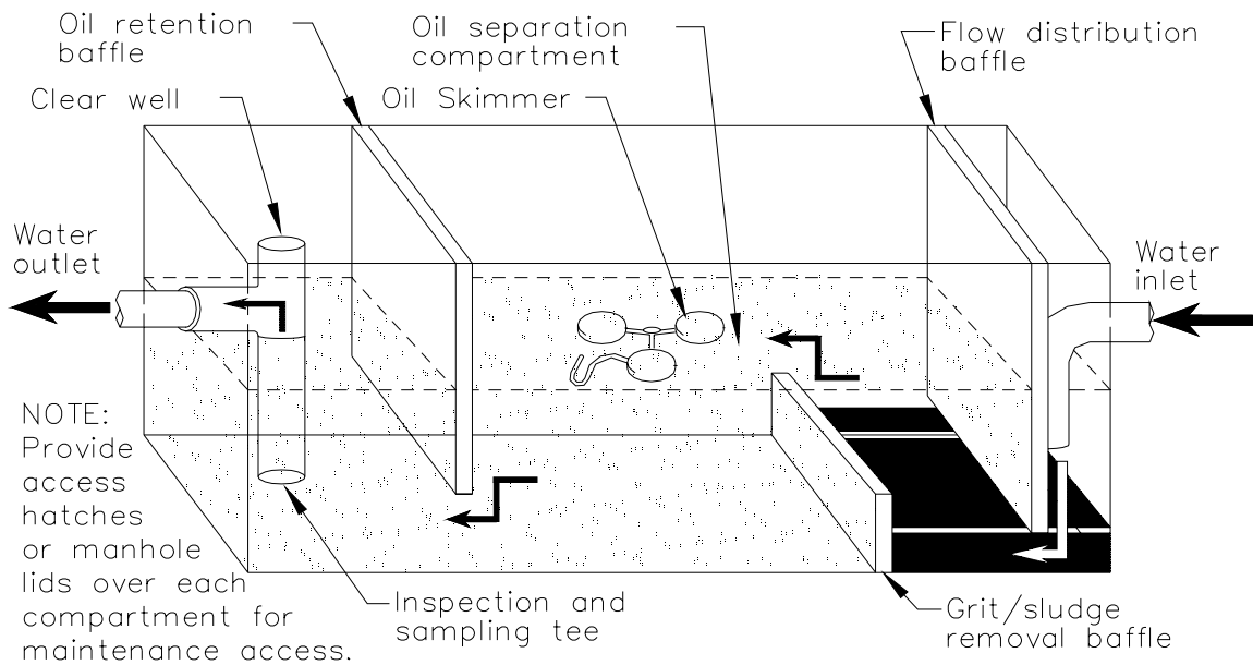
CONVENTIONAL SEPARATOR
