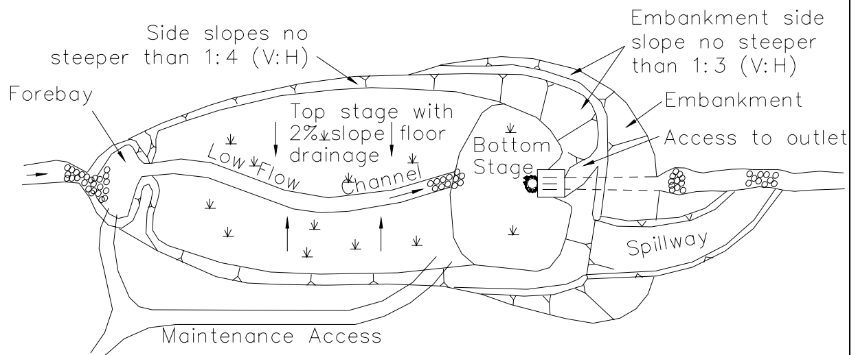
PLAN NTS
