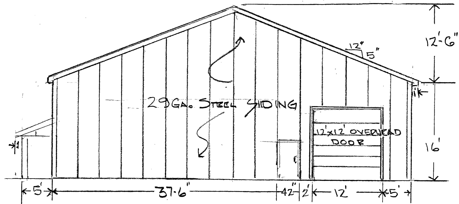
EAST ELEVATION
